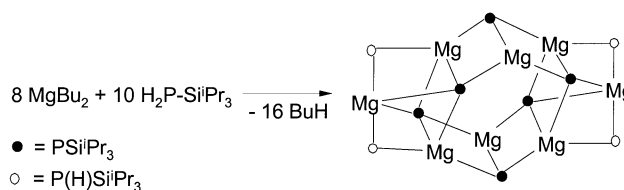
Scheme 2. Synthesis of 1
